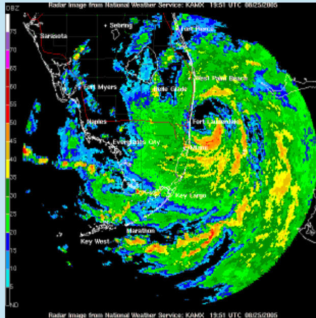
Hurricane Katrina nearing landfall over south Florida (Miami Radar image)
