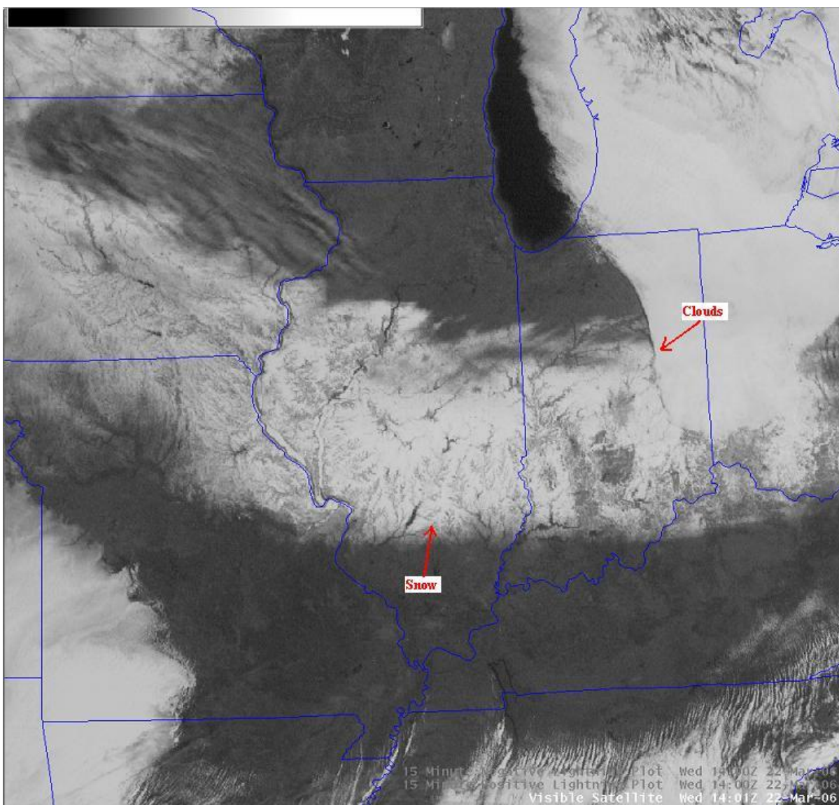
Visible Satellite picture showing the snowfall over the region on Wednesday morning, March 22 nd , 2006.
