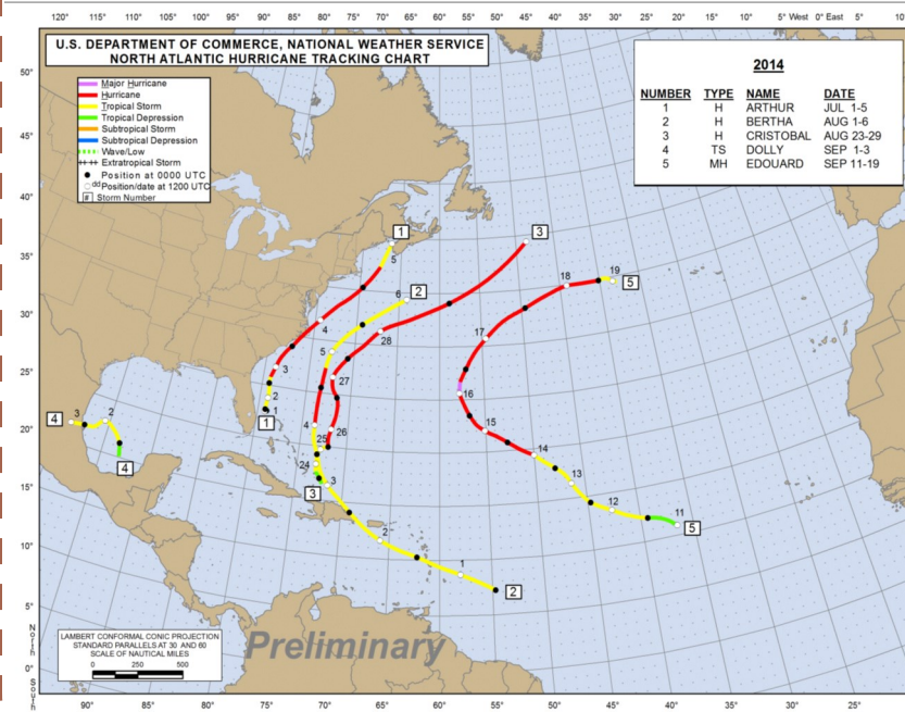
Above: Current Hurricane Tracks for the 2014 season. (Credit: National Hurricane Center)
